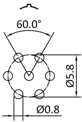
PCB OPEN SIZE(STRAIGHT)
