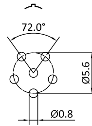
PCB OPEN SIZE(STRAIGHT)
